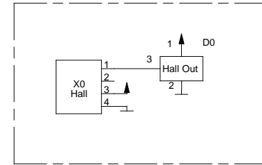
Hall PCB
