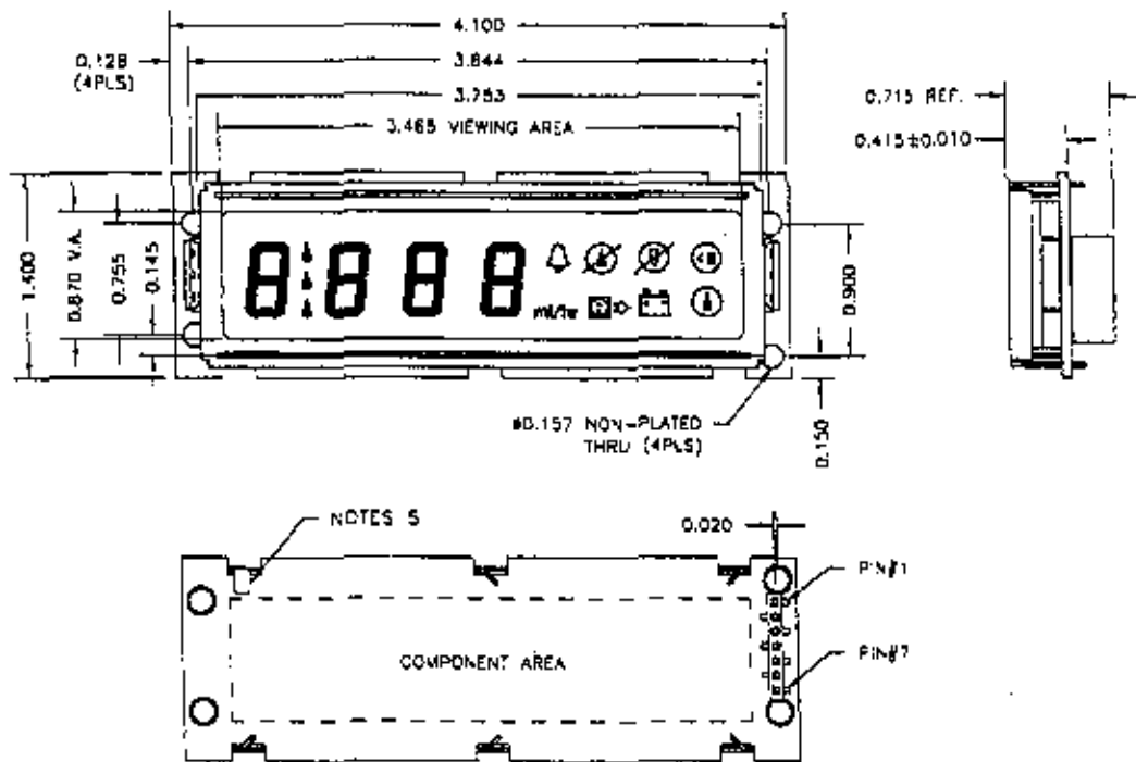
Figure 7-13, International Display Board Assembly
