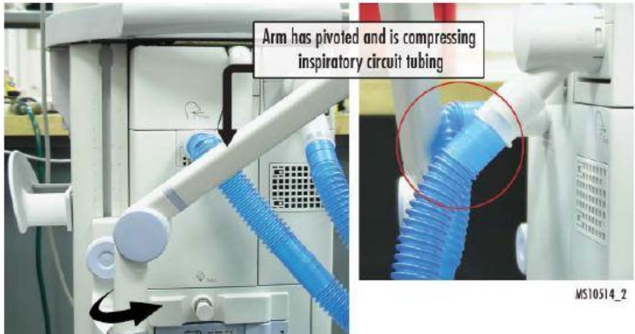
Figure 2. The arm has pivoted inward toward the cart and is compressing the circuit's inspiratory limb. This is possible because the articulating joint is below the level of the inspiratory port. If the joint is kept above the level of the port, this problem cannot occur. Another option is to mount the support arm on a different side of the ventilator, but this may not always be feasible.
